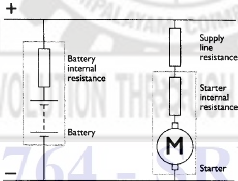
Equivalent circuit for a starter system
