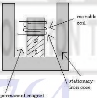
Fig 2. Voice coil
