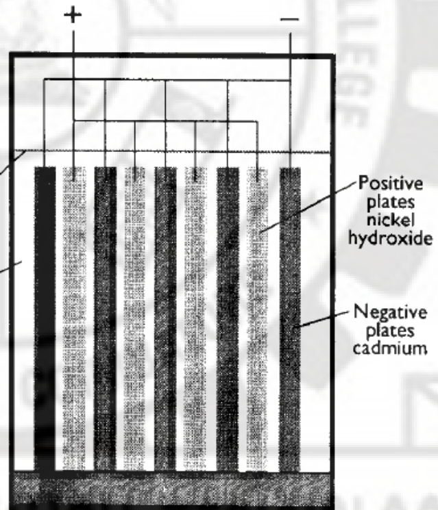
Figure 5.10 Simplified representation of a Nicad alkaline battery cell
