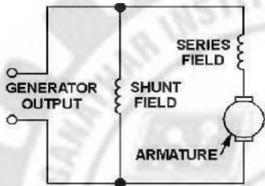
Compound wound long shunt
