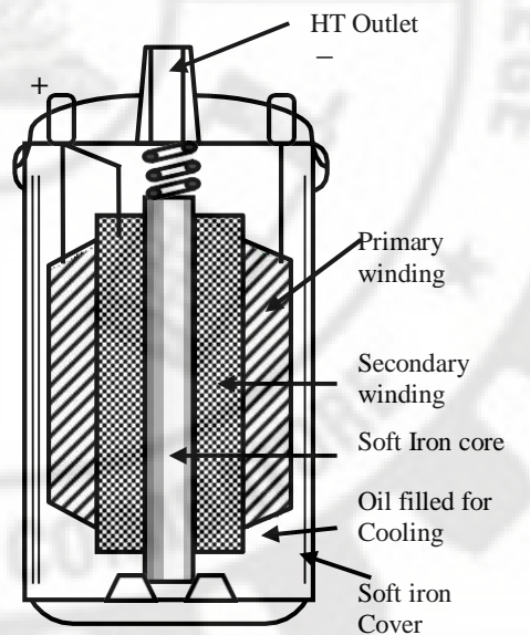
Ignition Coil
