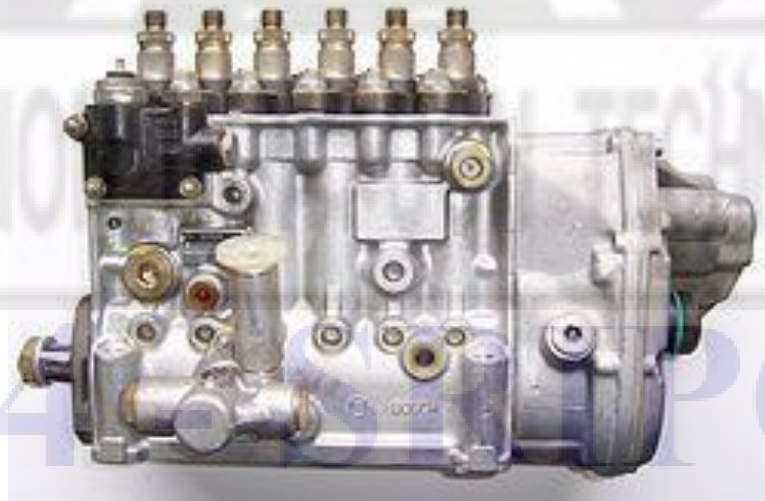
EDC injection inline pump
