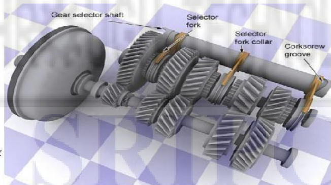
Fig. Electro-Hydraulic Manual Transmission
