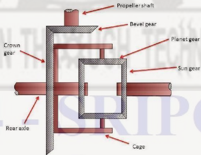
Differential gear
