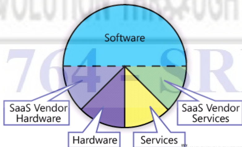
Fig 2.8 SaaS utilization
