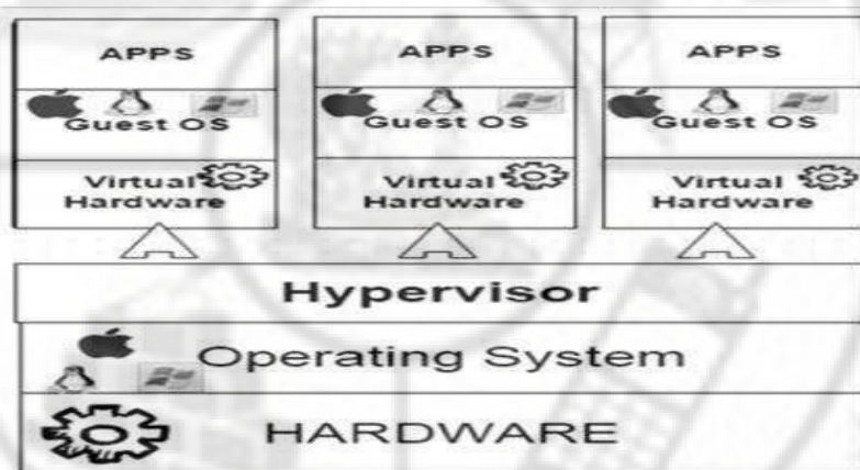
Figure 5.7: Virtual Threats
