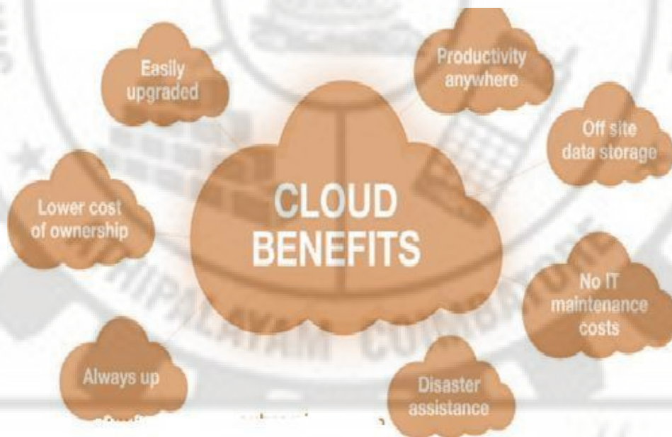
Fig 1.6 Cloud Benefits
