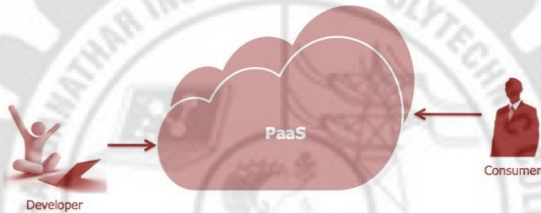
Fig 2.9 Paas users
