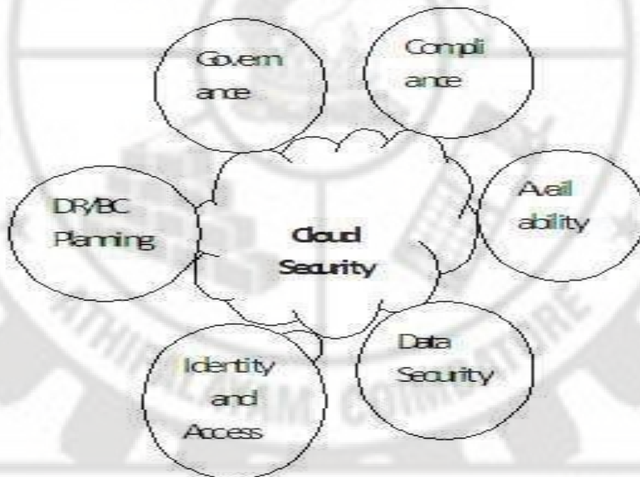
Fig 5.1 Cloud Security
