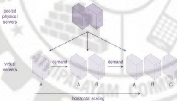
Fig 1.3 Horizontal Scaling
