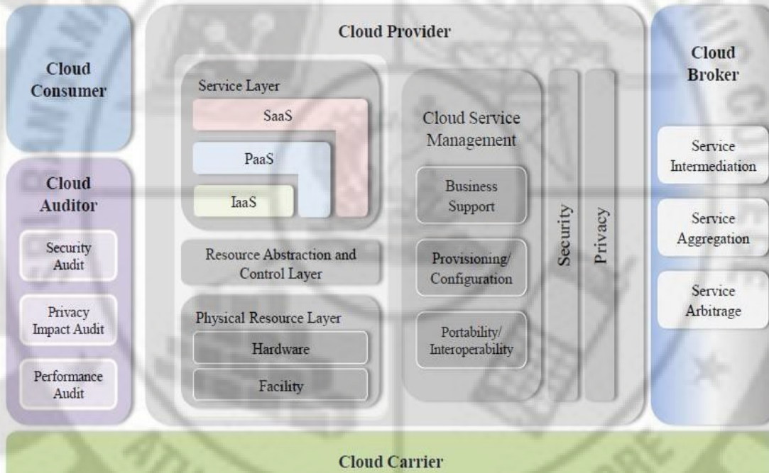
Fig 2.1 Cloud Architecture
