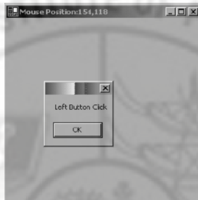
Fig. 3.32 Mouse Down
