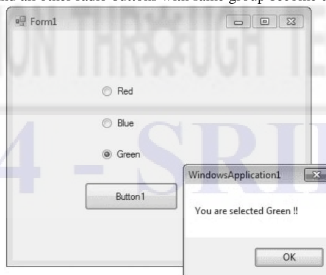
Fig. 3.12 Radio Button
