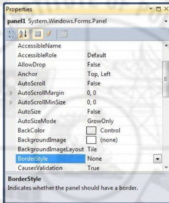
Fig. 3.27 Panel properties
