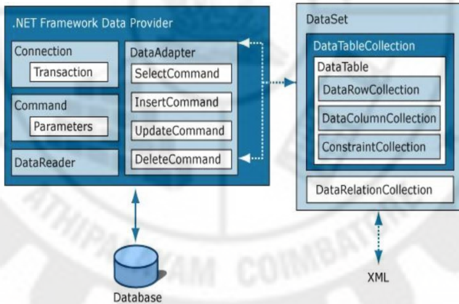
Figure 4.1: ADO.NET Architecture
