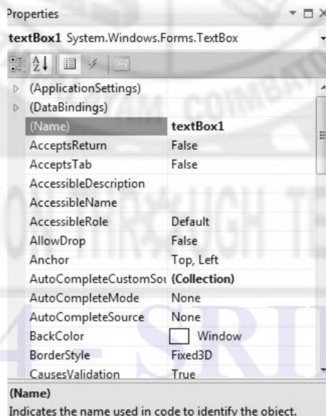
Fig. 3.9 Properties Window
