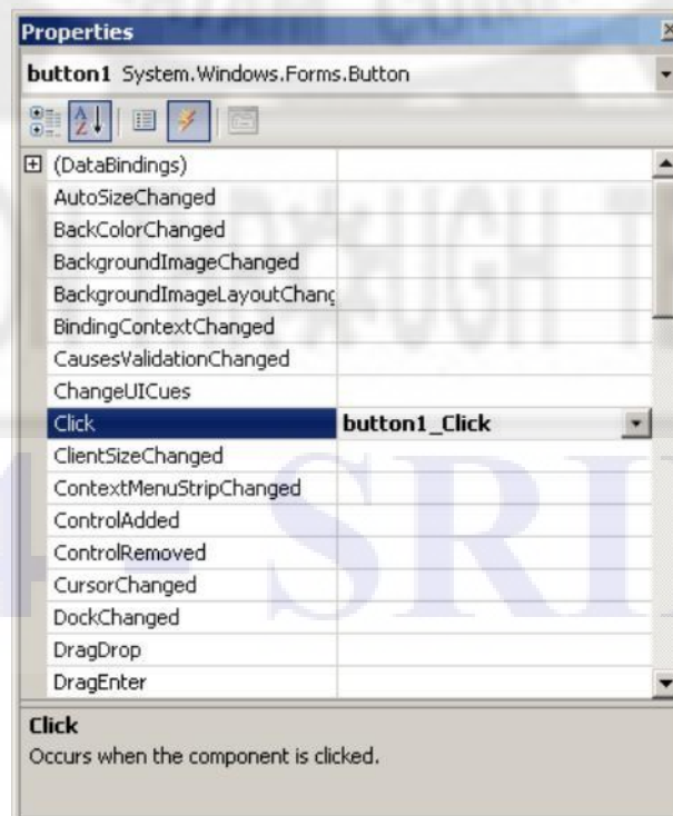
Fig.3.30 Button Events
