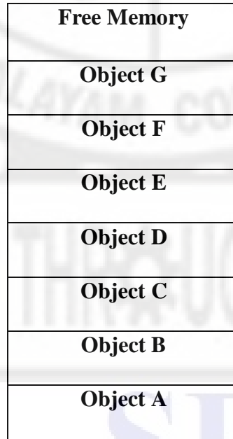
Figure 1.2 Managed Heap
