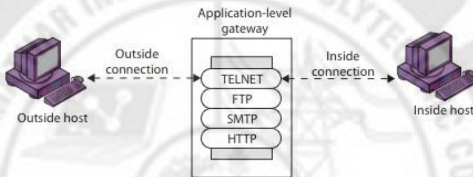
(b) Application-level gateway
