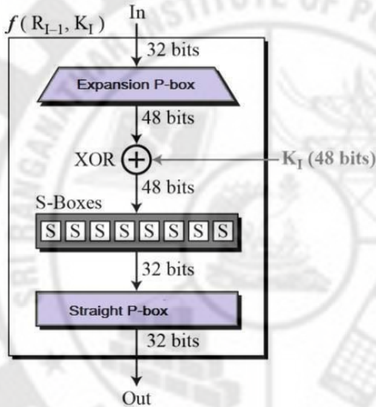
Fig 4.3 : ROUNDFUNCTION
