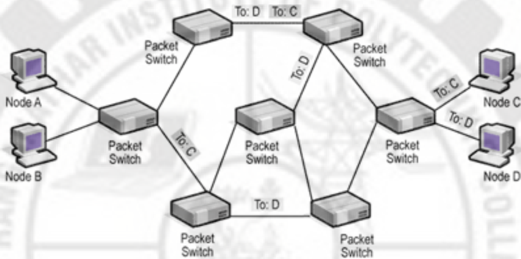
Fig 2.9 : Packet-Switched Networks
