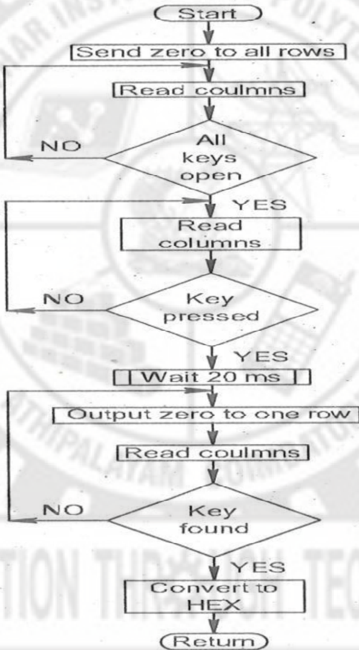
Fig 5.19 flow chart for keyboard scanning subroutine
