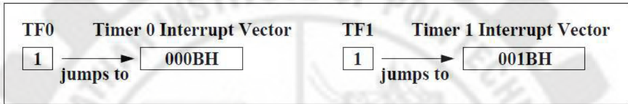
Fig 4.13 TF Interrupt
