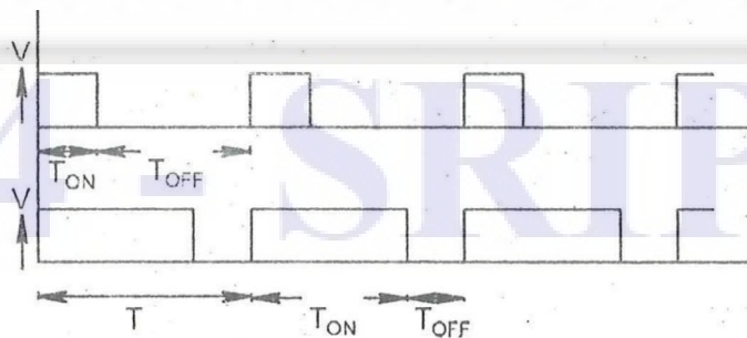
Fig 5.25 PWM signals
