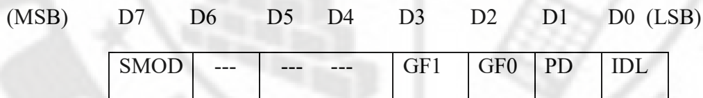
Fig 4.10 PCON Register
