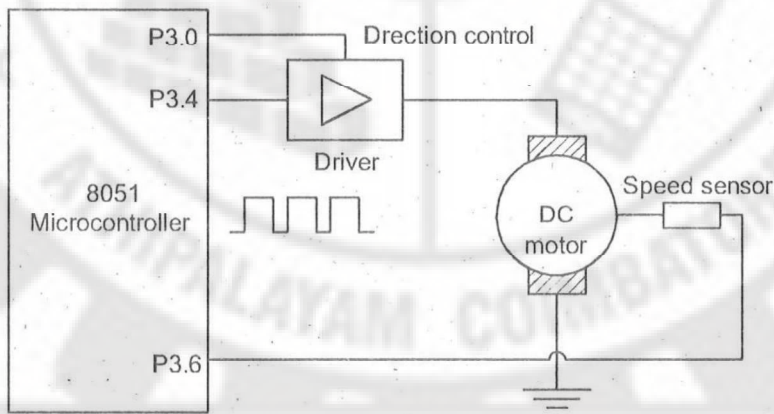
Fig 5.26 Interfacing diagram of DC motor 8051
