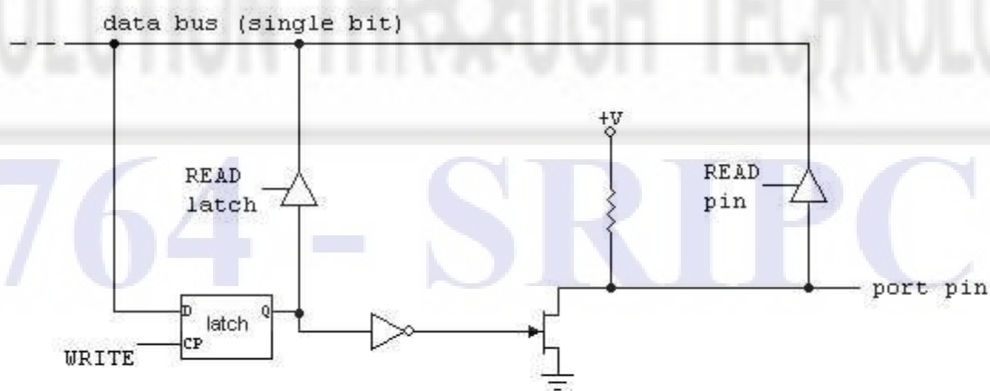
8051 single port pin
