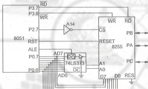
Fig 5.10 : 8051 Connection to the 8255
